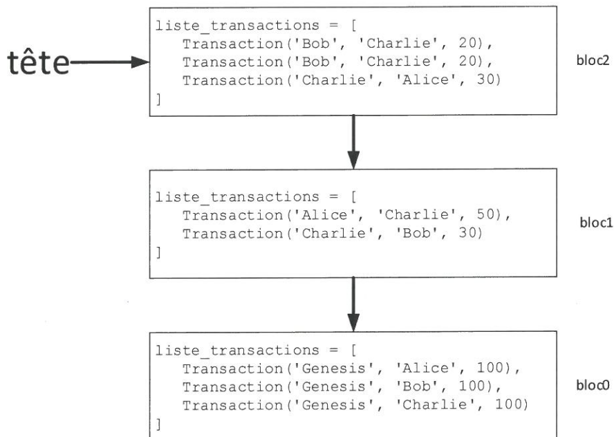
Figure 1. Blockchain
